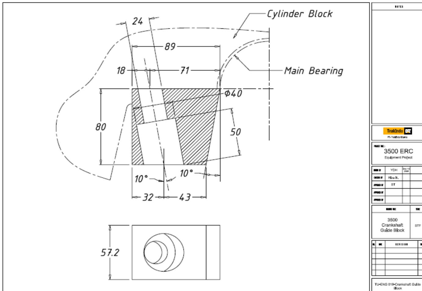
Figure 5: Drawing of guide block to be fabricated.
